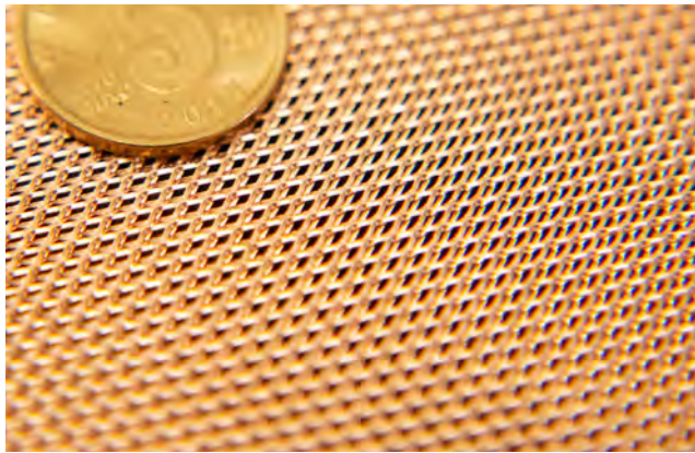
The copper and aluminum expanded metal foils is widely used on the composite blade material manufacturing for lightning striking protection, preventing the damage from lightning striking and extending the blade service life.
