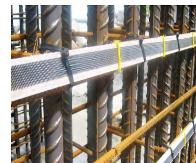
Cathodic Protection
